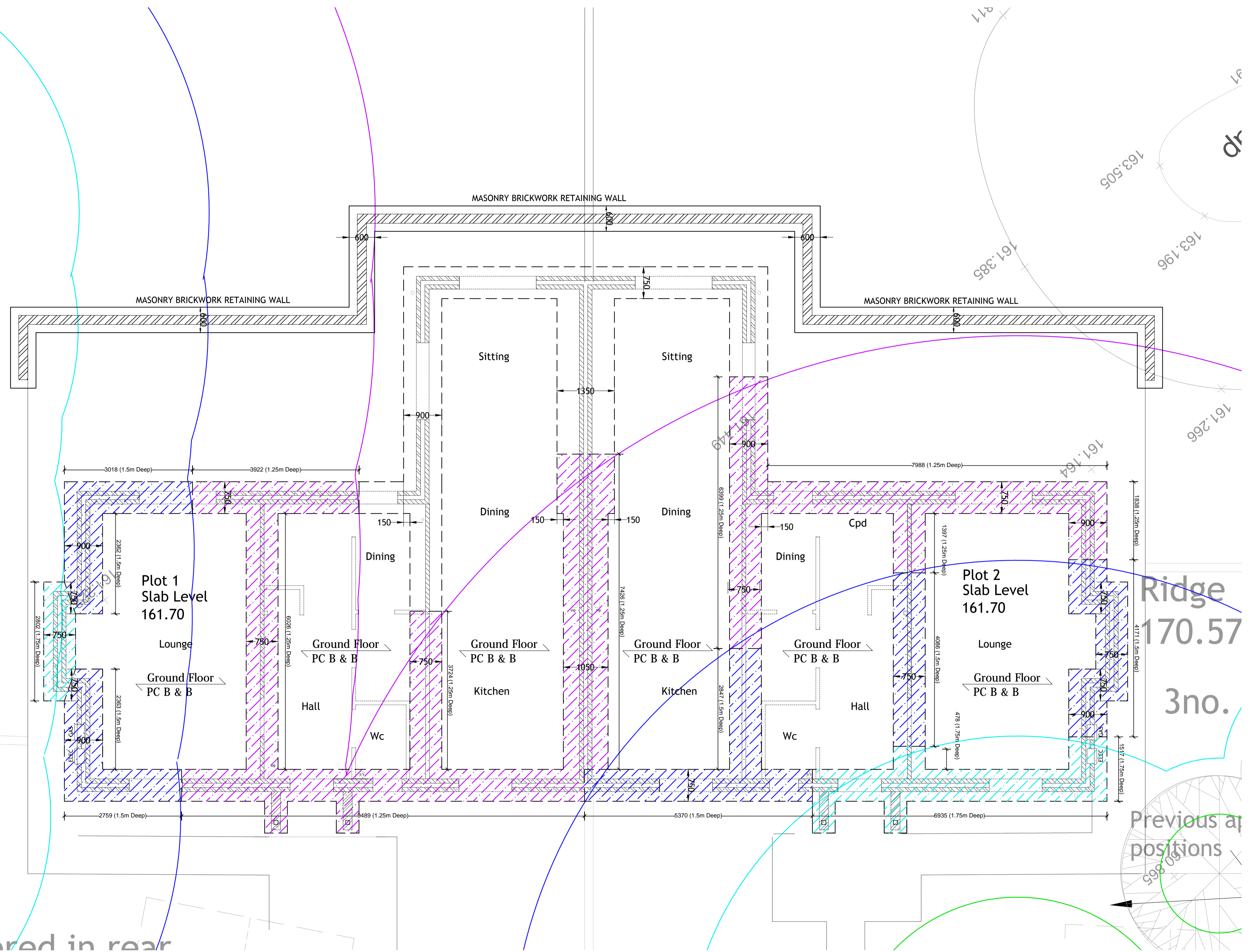
PLOTS 1 & 2 - FOUNDATIONS & GROUND FLOOR SPANS
