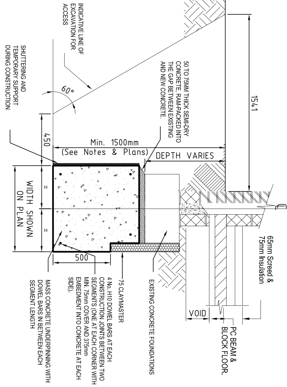
EXTERNAL WALL UNDERPINNING SCALE 1:25
