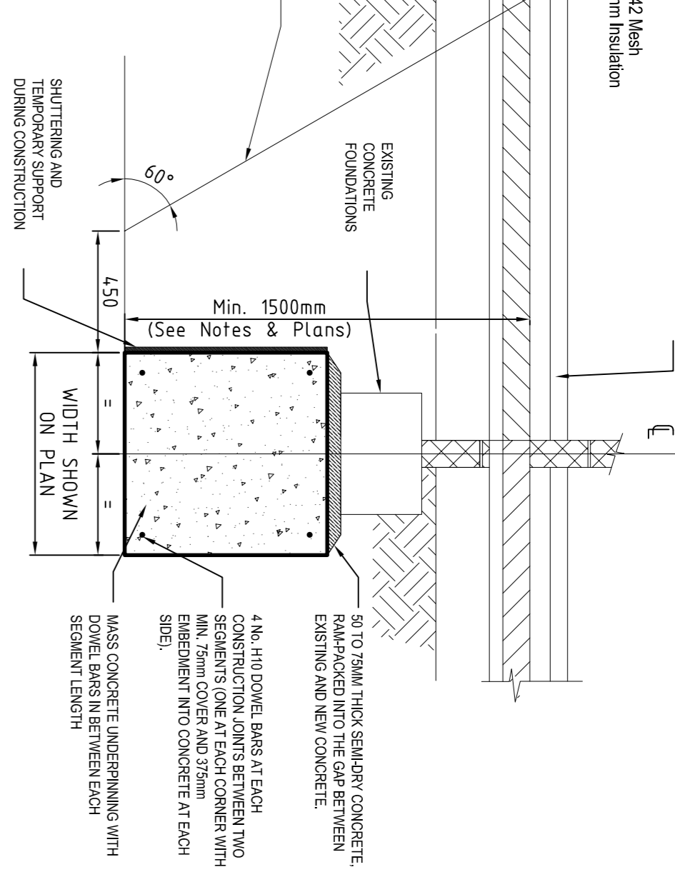
INTERNAL WALL UNDERPINNING SCALE 1:20
