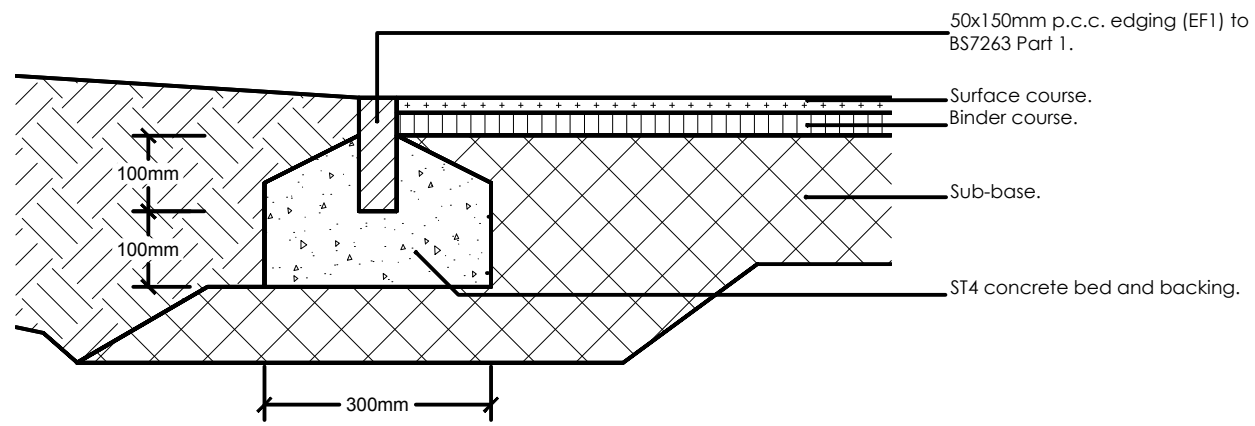
Pre-Cast Conc. Square Top Edging (EF1)
