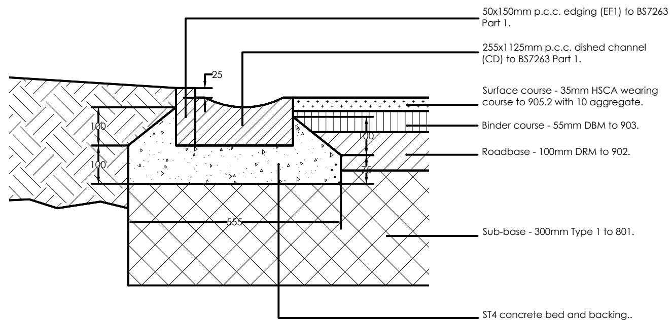
Pre-Cast Conc. Square Top Edging & Dished Channel (EF1CD)
