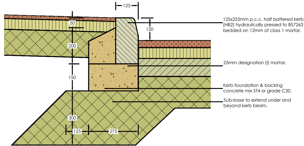
Half Battered Kerb Restraint (HB2)
