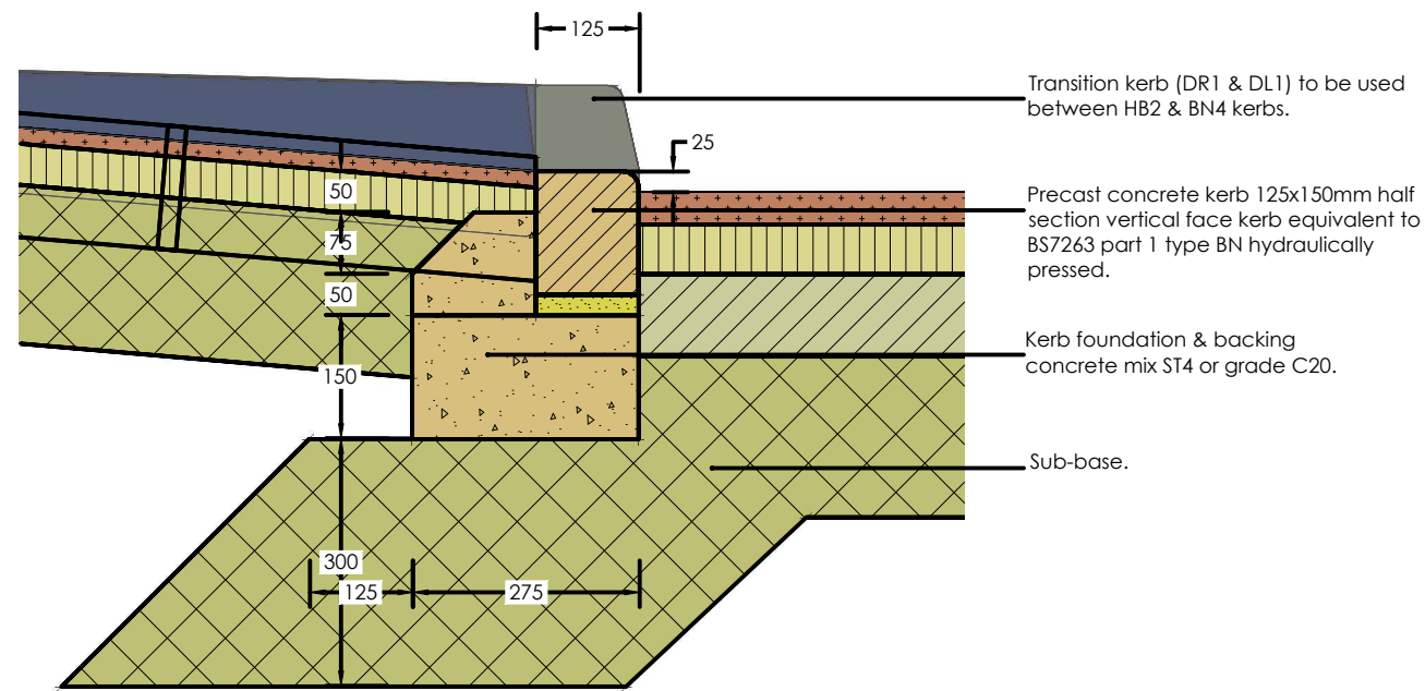
Bullnose Crossover Kerb (BN4)
